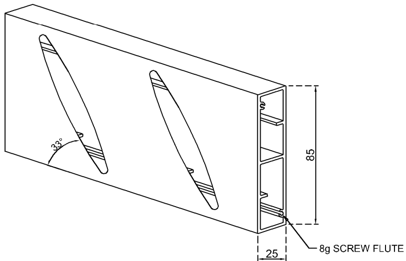
85mm x 25mm SLOTTED SIDE FRAME
